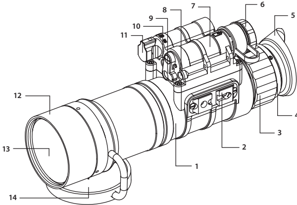
FIGURE 2-1. AVENGER NIGHT VISION MONOCULAR
