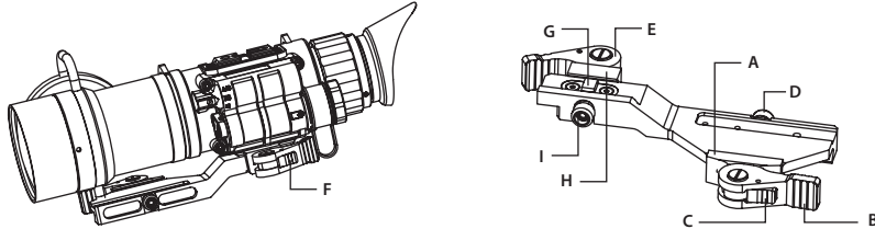
FIGURE 3-2. MOUNTING THE AVENGER TO A WEAPON WITH A QUICK-RELEASE PICATINNY MOUNT ADAPTER
