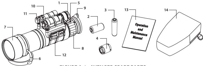
FIGURE A-1. AVENGER SPARE PARTS
