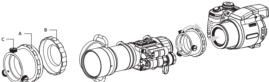
FIGURE 3-5. MOUNTING A CAMERA/ CAMCORDER TO THE AVENGER
