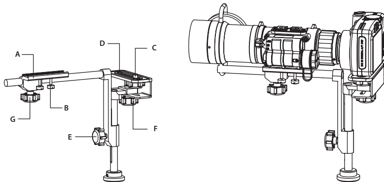
FIGURE 3-6. UNIVERSAL CAMERA ADAPTER APPLICATION
