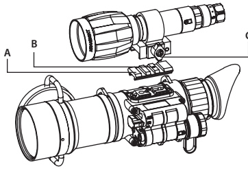
FIGURE 3-3. MOUNTING AN IR ILLUMINATOR TO THE AVENGER
