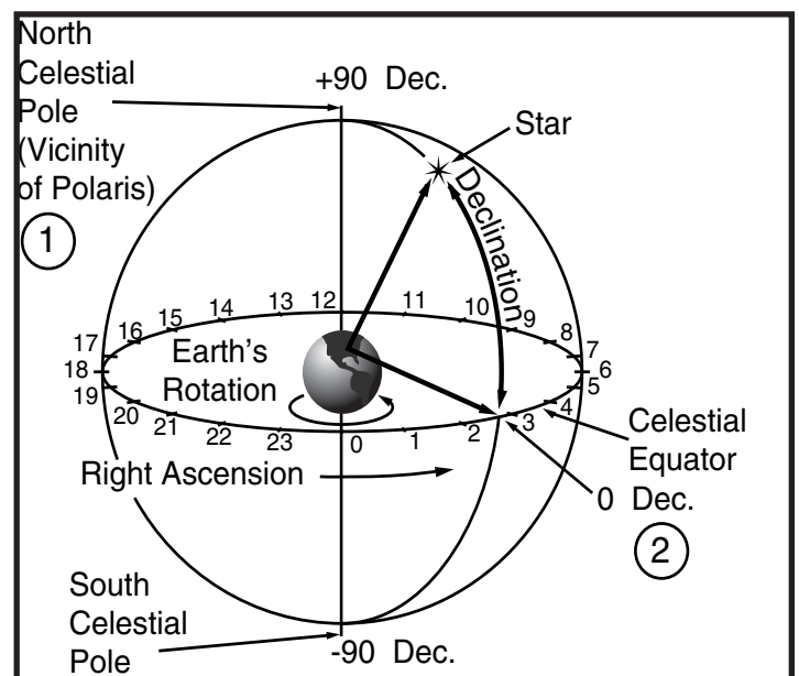
Figure 41: Celestial Sphere
