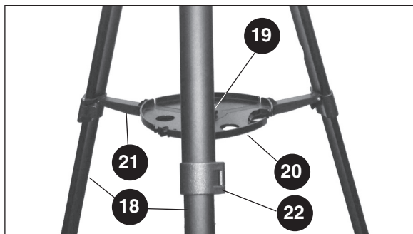
Fig. 2e (Inset): Tripod Assembly.
